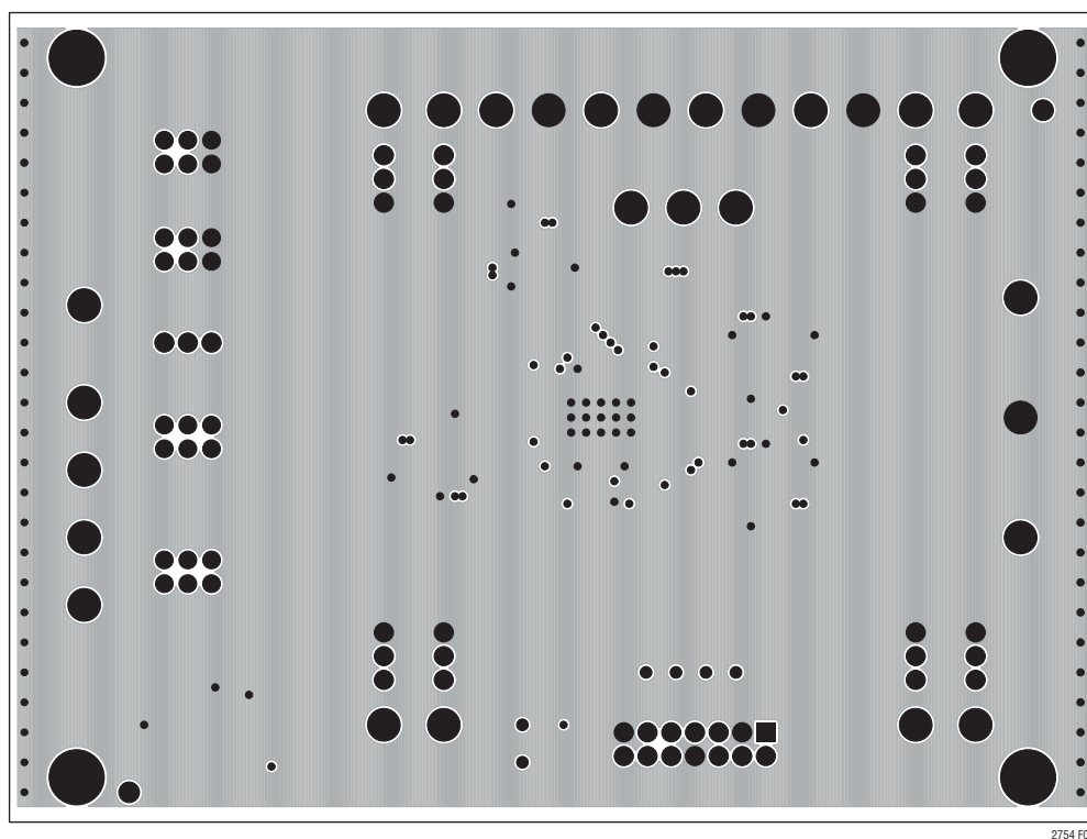
Figure 7. LTC2754 Evaluation Board DC1546. Layer 2, GND Plane
